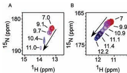
Figure 3. Overlay of series of ^1\text{H} – ^{15}\text{N} HSQC spectra of H \delta 1–N \delta 1 cross peak for (A) Ht cyt c_{552} wild type and (B) Ht -M13V/K22M at increasing pH values (arrow). In wild-type the chemical shift begins changing at a lower pH value than that of Ht -M13V/K22M.
