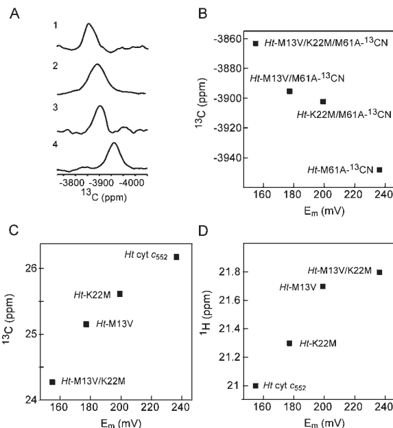
Figure 4. (A) 1–D ^{13}\text{C} spectra for (1) Ht -M13V/K22M/M61A- ^{13}\text{CN} , (2) Ht -M13V/M61A- ^{13}\text{CN} , (3) Ht -K22M/M61A- ^{13}\text{CN} , and (4) Ht -M61A- ^{13}\text{CN} . (B) Plot of ^{13}\text{C} cyanide chemical shift of the ^{13}\text{CN} derivative of Met-to-Ala variants vs reduction potential for Ht cyt c_{552} variants. (C) Plot of His16 ^{13}\text{C}\beta chemical shifts vs reduction potential for Ht cyt c_{552} variants. (D) Plot of average heme methyl ^1\text{H} chemical shifts vs reduction potential for Ht cyt c_{552} variants.
