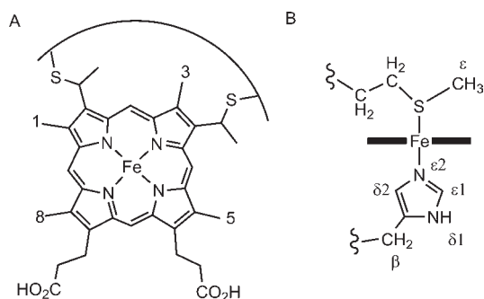
Figure 2. (A) Heme c , with heme methyls 1, 3, 5, and 8 labeled. (B) His and Met nomenclature conventions used herein.
